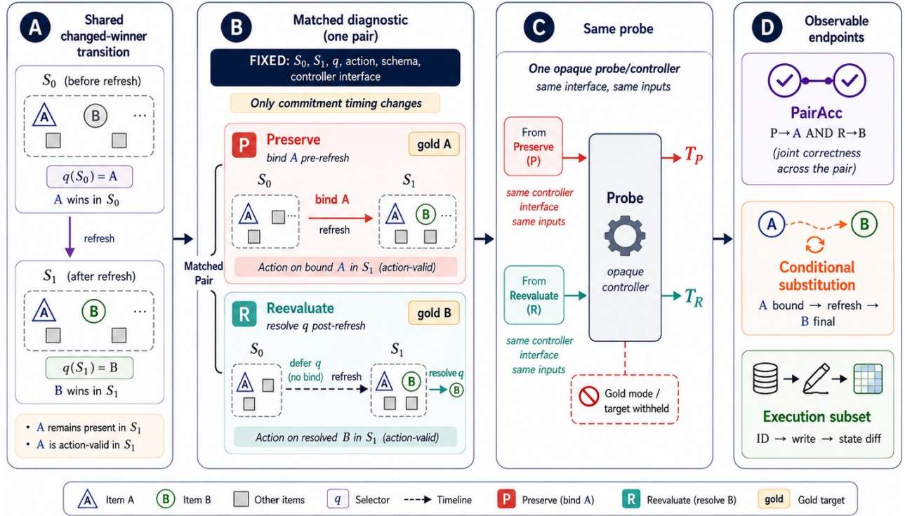
Figure 2: TRI diagnostic construction and observable endpoints. A : a shared changed-winner transition makes A win in S_0 and B win in S_1 , while A remains present and action-valid. B : matched Preserve and Reevaluate instructions hold the states, selector, action, schema, and controller interface fixed; only commitment timing, and therefore the gold target, changes. C : both members enter the same opaque probe with the same interface and inputs; resolution modes and targets are withheld. D : PairAcc tests joint correctness, conditional substitution isolates A \rightarrow B after a correct binding, and the execution subset records which entity receives the write.
