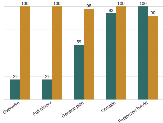
Qwen3.5
