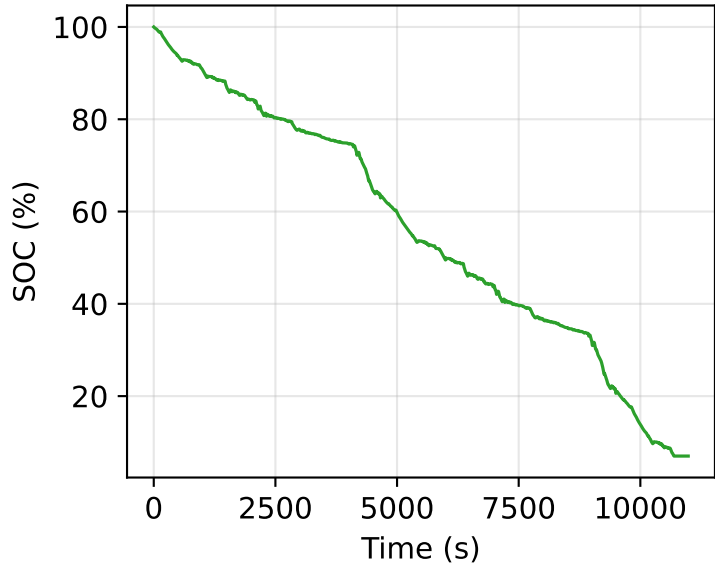
3. State of Charge Depletion
