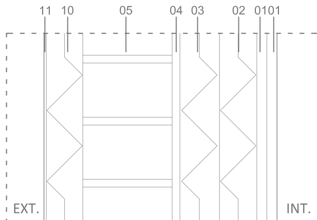
F02: FACHADA CHAPA
