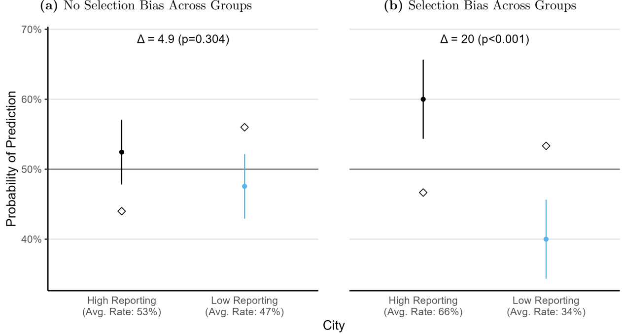
Figure 5: Prediction bias across groups
