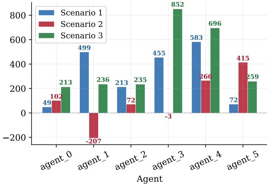
Cumulative reward per agent
