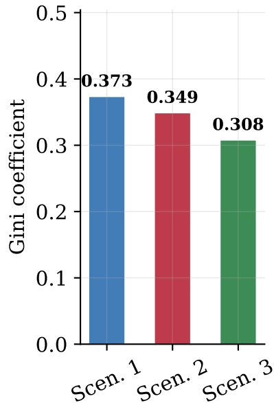
Gini index
