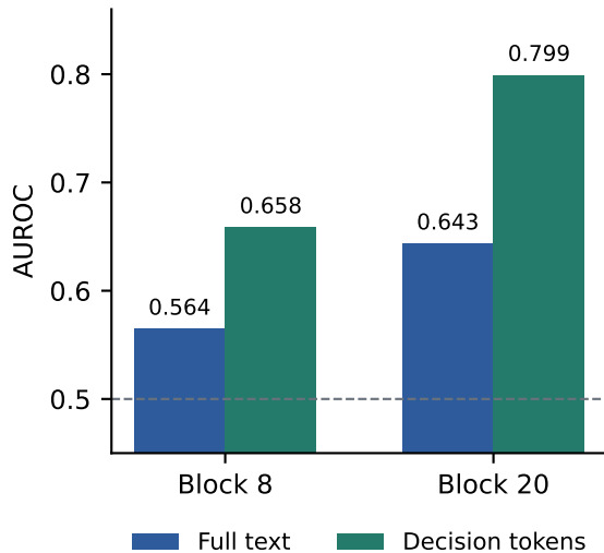
B. Matched lexicon isolates decision clauses
