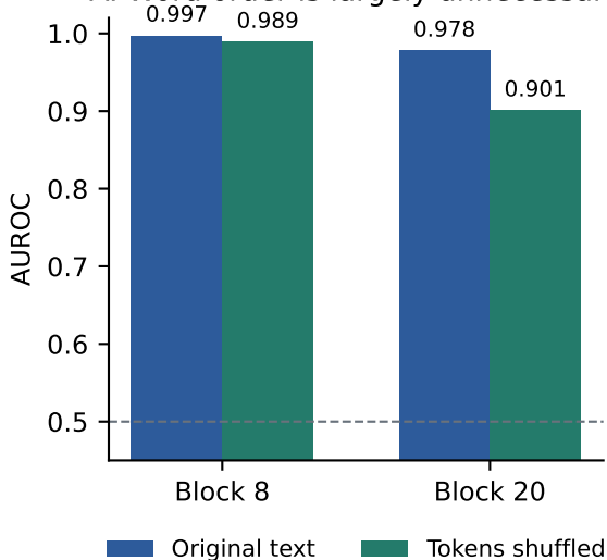
A. Word order is largely unnecessary
