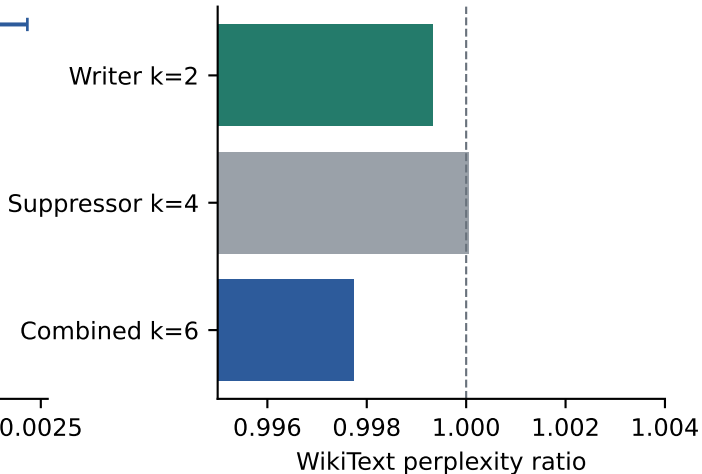
B. 45,338 held-out tokens
