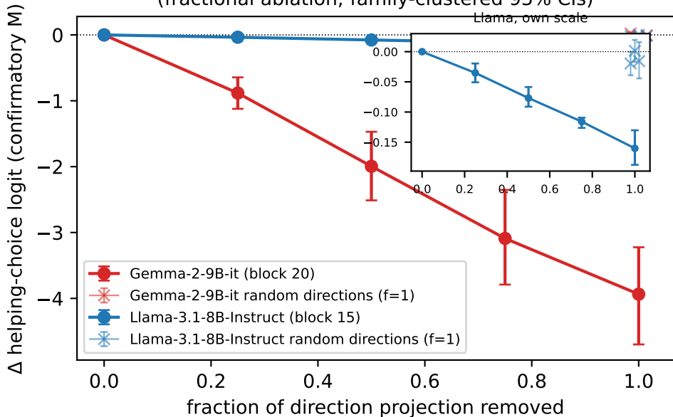
Direction dependence of the helping choice (fractional ablation; family-clustered 95% CIs)
