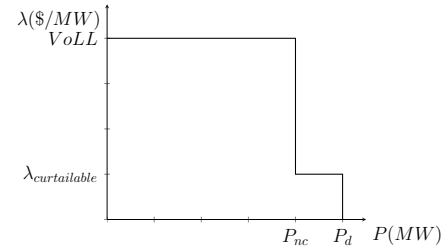
Fig. 3: Bid Function or Marginal Benefit of Dispatchable Loads.
