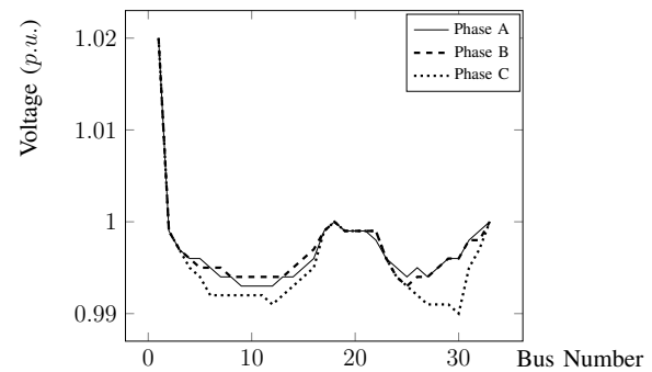
Fig. 5: Voltage Profile of Unbalanced Three-phase Test System in Radial Configuration.
