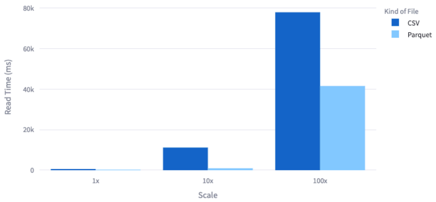
CSV vs Parquet Read Time Across Different Scales
