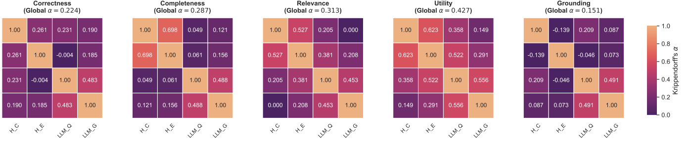
Figure 7: Judges agreement computed using the Krippendorff’s \alpha .
