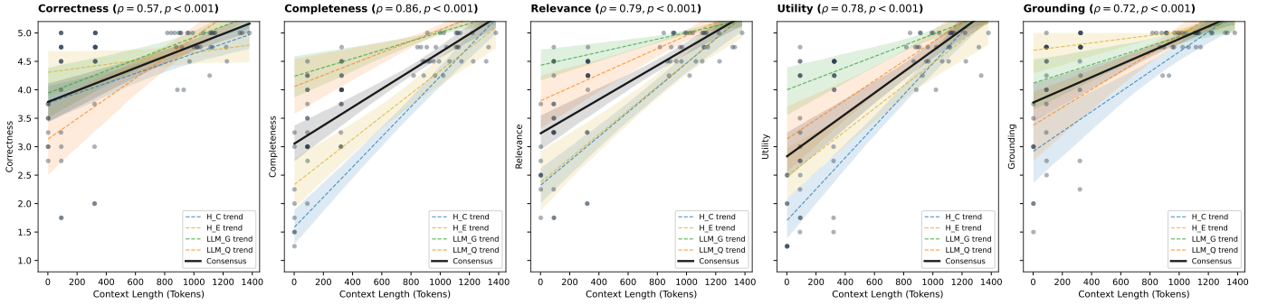
Figure 8: Evaluation scores against the available context length in tokens for all 4 judges plus the consensus (average).
