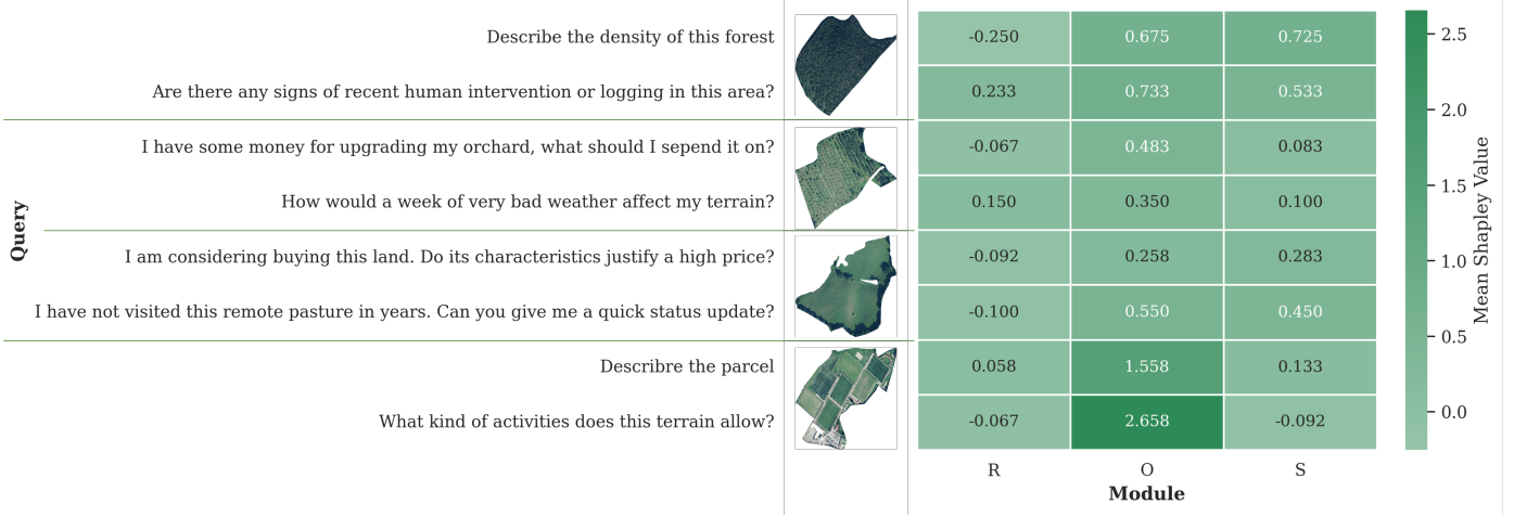
Figure 6: Shapley values by query aggregating across judges and metrics.
