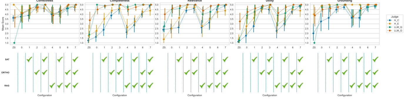
Figure 4: Evaluation results from the Ablation Study phase for the 4 evaluators and 5 metrics grouped by configuration. Differences can be observed based on active modules.
