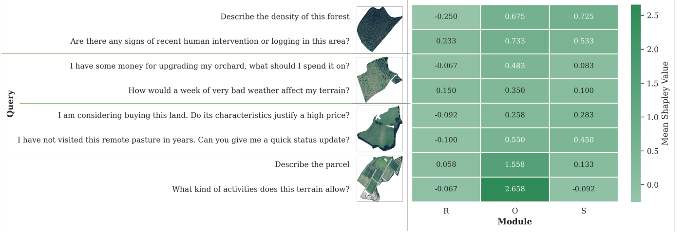
Figure 7: Shapley values by query aggregating across judges and metrics.
