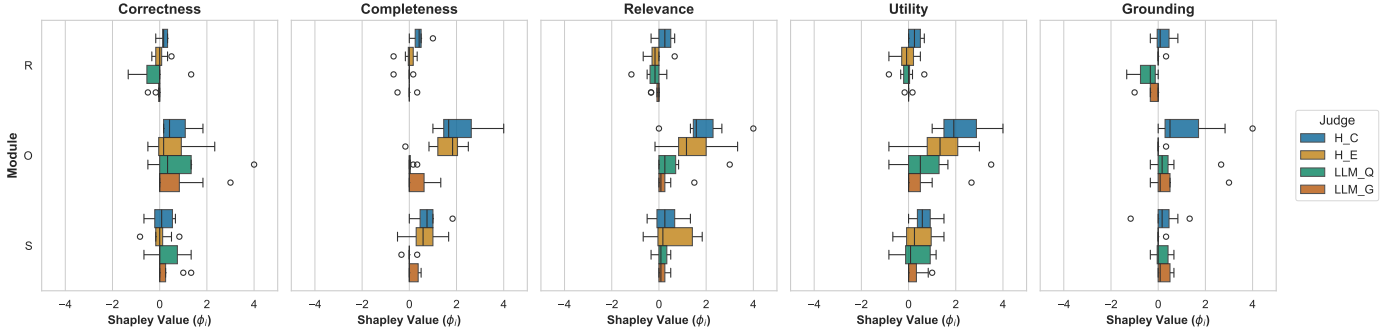
Figure 6: Marginal contributions of each module R, O, S quantified with the Shapley values \phi_i across the panel of 4 judges and the 5 metrics. Each box summarises the eight ablation queries ( n=8 ). Confidence Intervals reported in Table A.5 of Appendix A.
