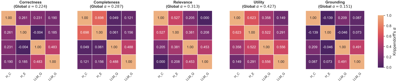
Figure 8: Judges agreement computed using the Krippendorff's \alpha (n=143).
