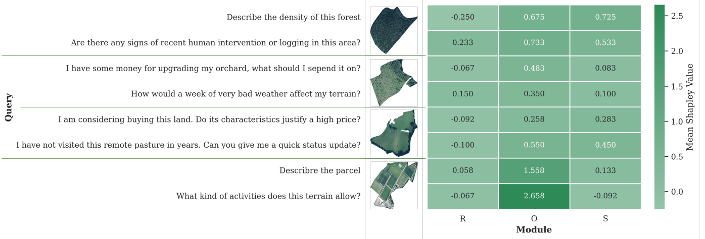
Figure 6: Shapley values by query aggregating across judges and metrics. Comentar colores blanco y negro del texto?
