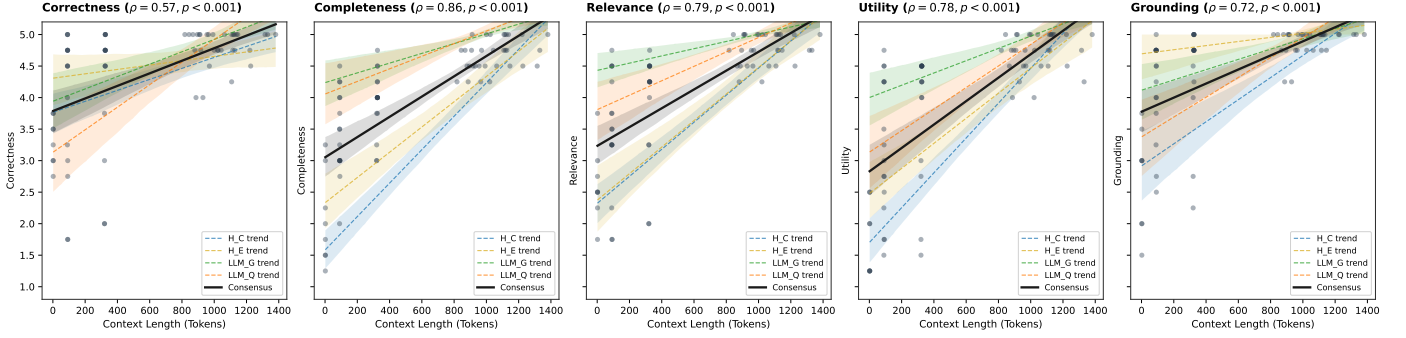
Figure 8: Evaluation scores against the available context length in tokens for all 4 judges plus the consensus (average).
