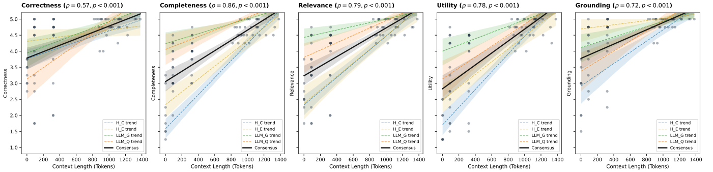
Figure 9: Evaluation scores against the available context length in tokens for all 4 judges plus the consensus (average).
