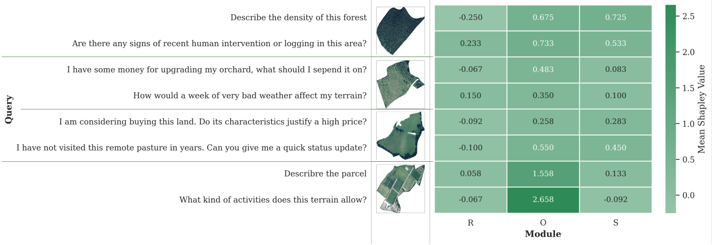
Figure 7: Shapley values by query aggregating across judges and metrics. Comentar colores blanco y negro del texto?
