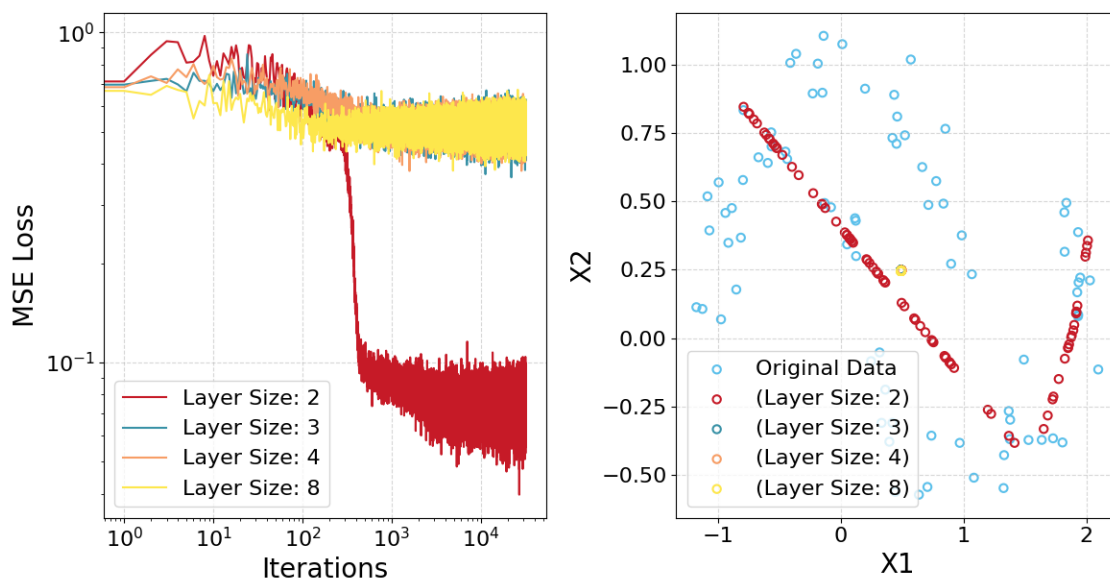
Autoencoder Training: Influence of Layer Size
