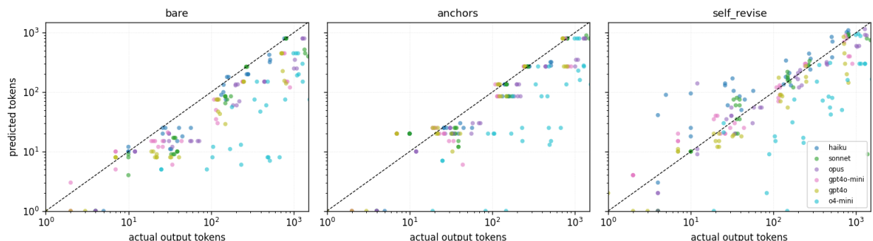
Figure 10: E6, per run: predicted vs. actual output tokens by condition, one dot per trial, coloured by model. The point cloud lifts toward the diagonal from bare to self_revise; the lone band that stays far below in every condition is o4-mini.
