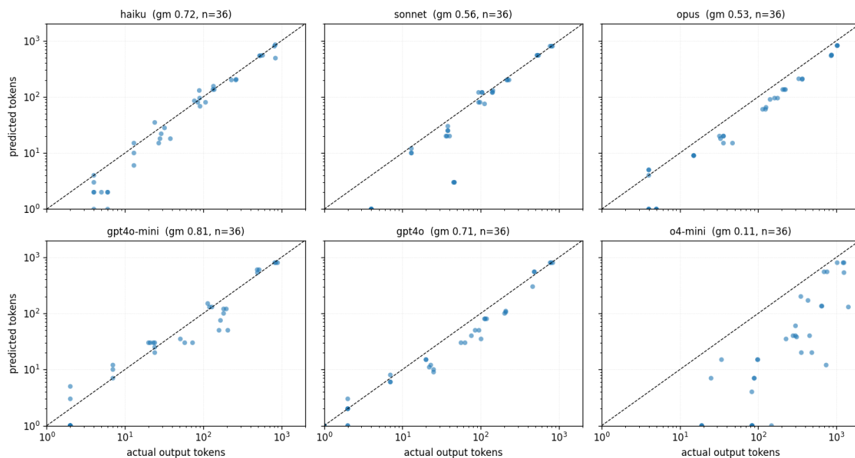
Figure 8: E2, per run: predicted vs. actual output tokens (token-estimate condition), one dot per trial, log-log, dashed line is perfect calibration. The consistent offset below the diagonal is the systematic \sim 2\times undershoot; o4-mini (a reasoning model) sits far below, undershooting roughly ten-fold.
