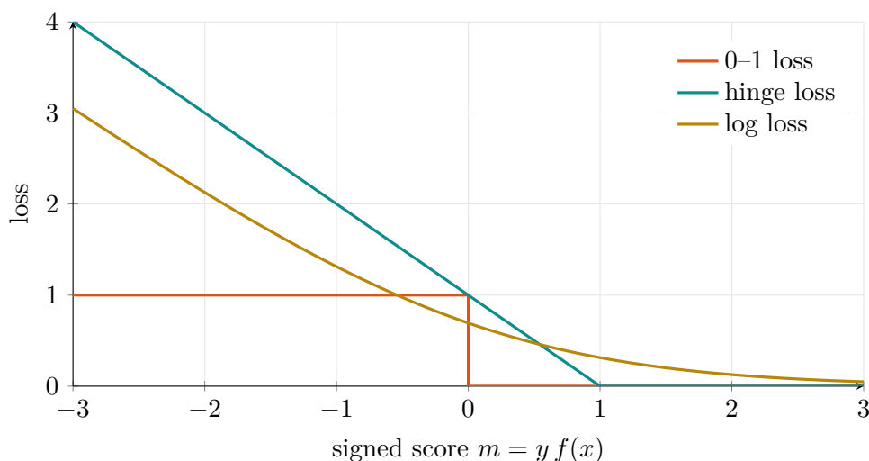
Figure 1: The three losses as functions of the signed score m = yf(x) . Positive m means a correct prediction. Unlike the 0–1 loss, the hinge and the log loss have a slope that points towards fewer mistakes, and both are convex (bowl-shaped), which makes them easy to minimize.
