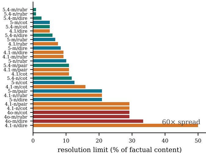
(a) what quality gap a judge can actually resolve
