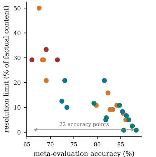
(b) accuracy compresses the difference
