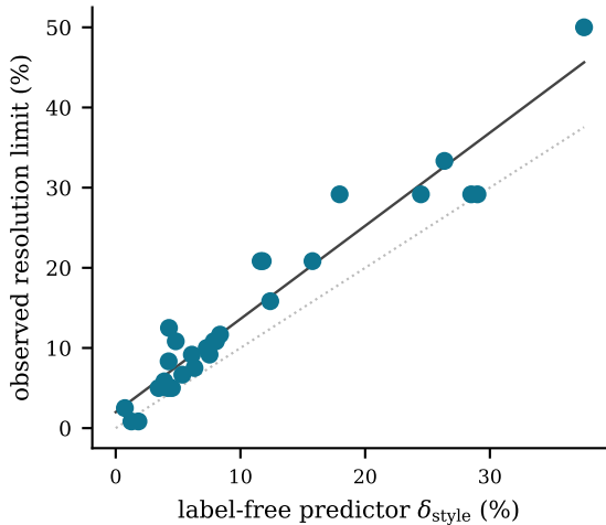
(a) label-free: R^2=0.927 , resid 3.2%
