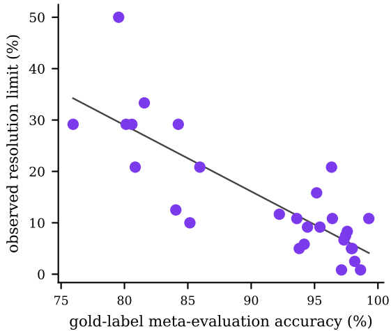
(b) gold-label: R^2=0.667 , resid 6.9%
