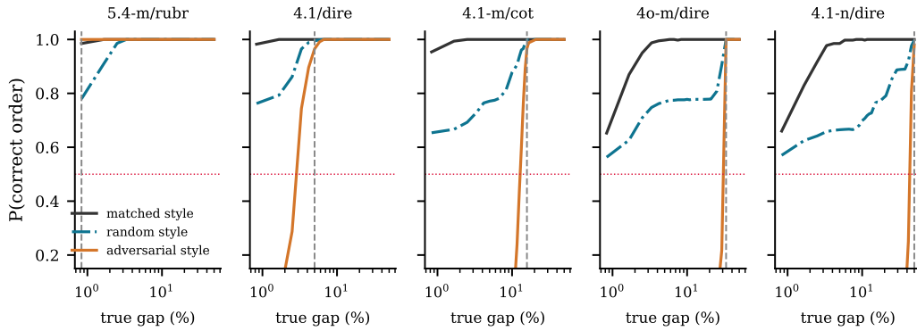
Figure 2: Probability of correctly ordering two systems as a function of their true quality gap (log axis), for five representative judges ordered by resolution limit. Black: both systems rendered in the same style. Teal: styles assigned independently at random. Orange: the worse system wears the judge’s preferred style. Dashed grey marks the measured resolution limit. Takeaway: the adversarial curve is a step, and its location—not the judge’s average accuracy—is what determines whether a leaderboard gap means anything.
