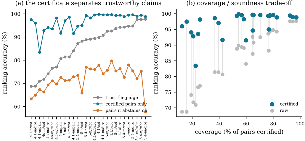
Figure 5: The certificate in the leaderboard regime (gaps \leq 16.7\% of factual content, independent styles). (a) Judges sorted by raw accuracy. (b) Coverage against accuracy. Takeaway: certified orderings are reliable across the whole judge pool, the pairs the certificate declines are exactly the unreliable ones, and weak judges correctly certify almost nothing.
