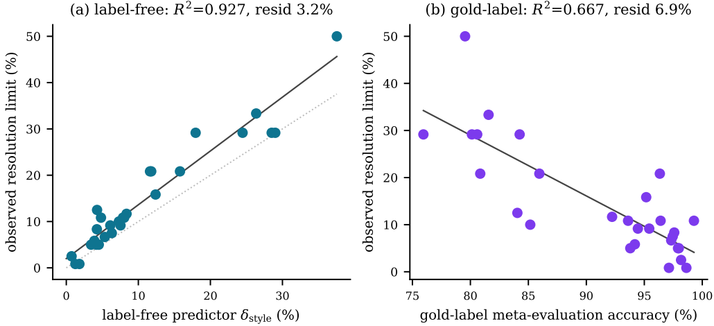
Figure 4: Recovering the resolution limit. (a) The label-free predictor \delta_{\text{style}} ; dotted line is y = x . (b) Gold-label accuracy on a clear-cut, style-matched meta-benchmark. Takeaway: both are informative, but only the label-free predictor is calibrated well enough to convert into a decision about a specific leaderboard gap.
