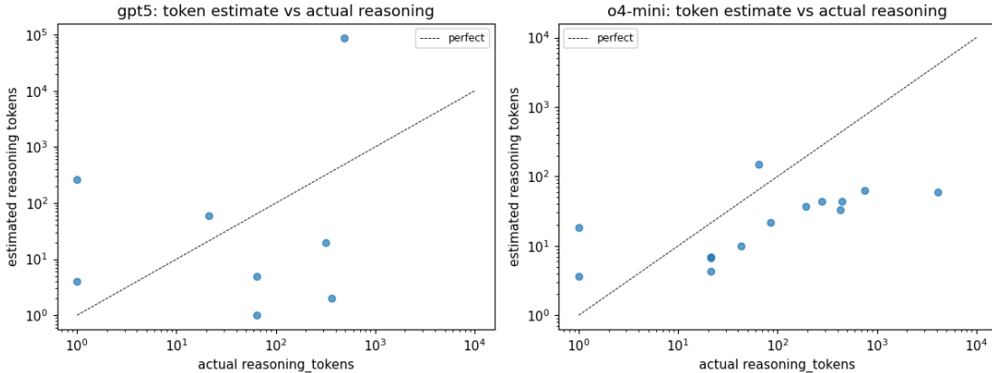
Figure 7: E10: predicted vs. actual reasoning tokens, log–log, per model. Estimates cluster in a narrow range relative to the wide spread of actuals — the model can rank but cannot size.
