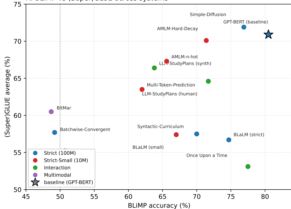
A. BLiMP vs (Super)GLUE across systems
