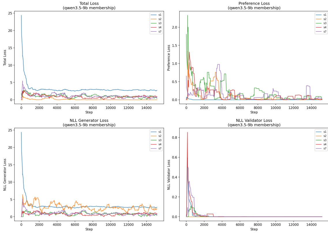
Figure 3: Training loss curves for Qwen3.5-9B on membership.
