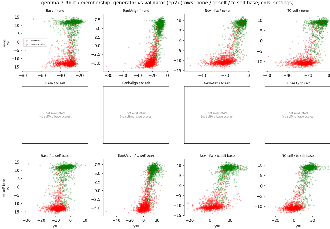
Figure 13: Generator vs validator scores, gemma-2-9b-it / membership, ep2 (member green, non-member red). Rows = generator scoring variant: none (raw log P ), tc self (own-model typicality), tc self base (base-model typicality); columns = settings . For these gemma-2-9b-it train-set evals only base-typicality was computed (self-typicality / own-model was run only for the held-out test sets, not the train set this scatter uses), so the tc self row has no train data and is marked “not evaluated”; only none and tc self base are available here. (The HumanEval per-problem train eval did include the own-model self mode, so its scatter has all three rows.)
