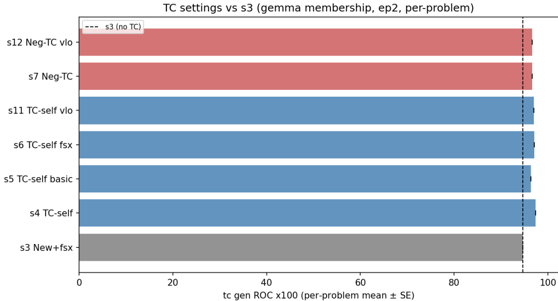
Figure 15: TC comparison on gemma membership (ep2): per-problem typicality-corrected gen ROC ( \times 100 , mean \pm SE) for the TC settings (self-TC: s4/s5/s6/s11; neg-TC: s7/s12) against the no-TC s3 baseline (dashed). Same per-problem procedure as the HumanEval report.
