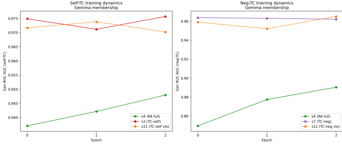
Figure 10: Epoch-by-epoch dynamics for TC comparison. TC-trained models converge quickly and maintain advantage throughout training.
