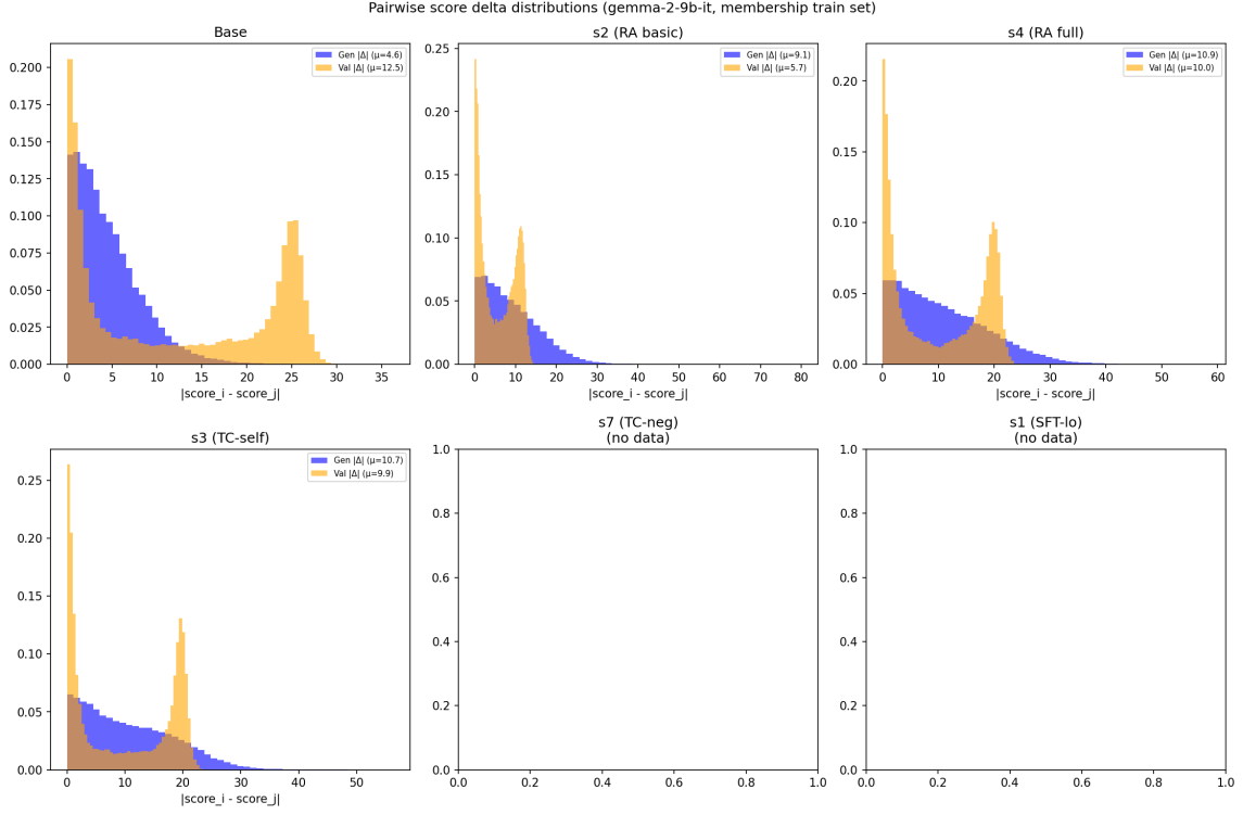
Figure 6: Pairwise score delta distributions for gemma membership. Generator (blue) and validator (orange) distributions. Tighter = better calibrated.
