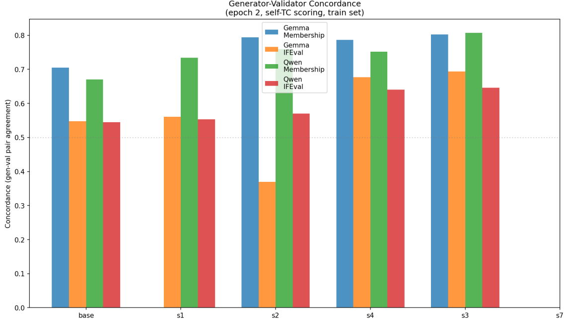
Figure 8: Concordance across all model/task combinations.
