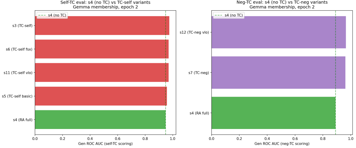
Figure 9: TC comparison: self-TC variants (left) and neg-TC variants (right) against s4 baseline.
