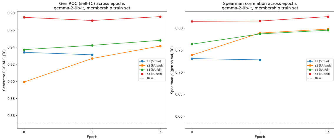
Figure 7: Training dynamics for gemma membership: Gen ROC and Spearman across epochs.
