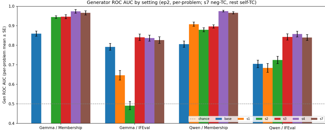
Figure 1: Generator ROC AUC across settings and model/task combinations (epoch 2, train set), per-problem mean with SE error bars . Self-TC scoring for all settings except s7 (neg-TC), scored with neg-TC to match its training-time TC type. Dashed line is chance (0.5).
