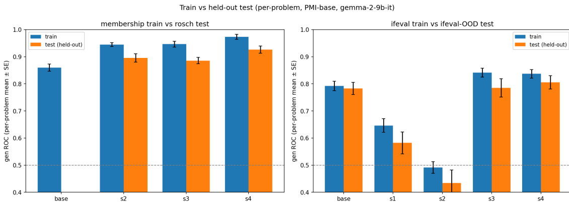
Figure 16: Train vs held-out test gen ROC, per-problem mean with SE error bars (PMI-base, gemma-2-9b-it). Left: membership train vs rosch test. Right: ifeval train vs ifeval-OOD test. Dashed line is chance. Same per-problem procedure as the rest of this report.
