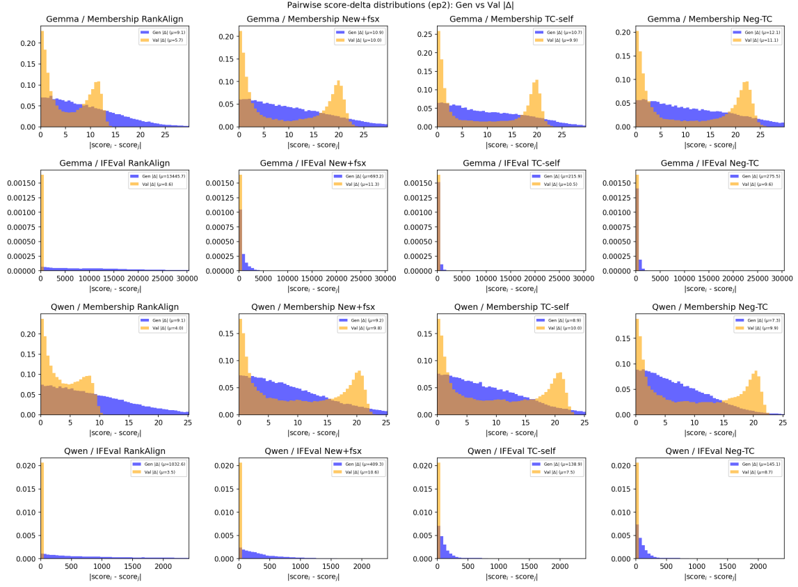
Figure 10: Pairwise score-delta distributions (ep2), the original report’s diagnostic: candidates are pooled per (model, dataset, setting) and \sim 100k random pairs sampled; each panel overlays |score_i - score_j| for the generator (blue, typicality-corrected) and validator (orange, log-odds), with mean \mu in the legend. Tighter = better calibrated; a long generator tail flags score-spread/instability (e.g. RankAlign s2 on IFEval).
