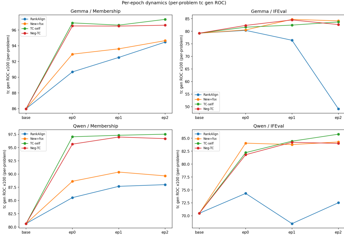
Figure 11: Per-epoch training dynamics: per-problem typicality-corrected gen ROC ( \times 100 ) vs. checkpoint (base/ep0/ep1/ep2) for s2/s3/s4/s7, each in its natural eval mode, across all four model/task cells. Same per-problem procedure as the HumanEval report. Note RankAlign (s2) on Gemma/IFEval collapses toward chance by ep2.
