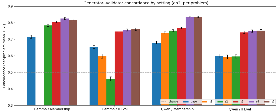
Figure 12: Generator-validator concordance by setting (ep2), per-problem mean with SE error bars , across all four cells. Dashed line is chance (0.5); s2 on Gemma/IFEval falls below it.
