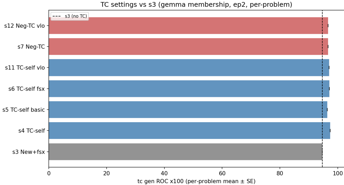
Figure 15: TC comparison on gemma membership (ep2): per-problem typicality-corrected gen ROC ( \times 100 , \text{mean} \pm \text{SE} ) for the TC settings (self-TC: s4/s5/s6/s11; neg-TC: s7/s12) against the no-TC s3 baseline (dashed). Same per-problem procedure as the HumanEval report.
