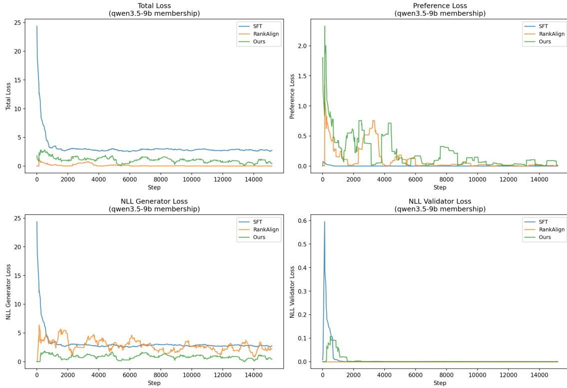
Figure 4: Loss curves: SFT vs RankAlign vs Ours (Qwen3.5-9B, membership).
