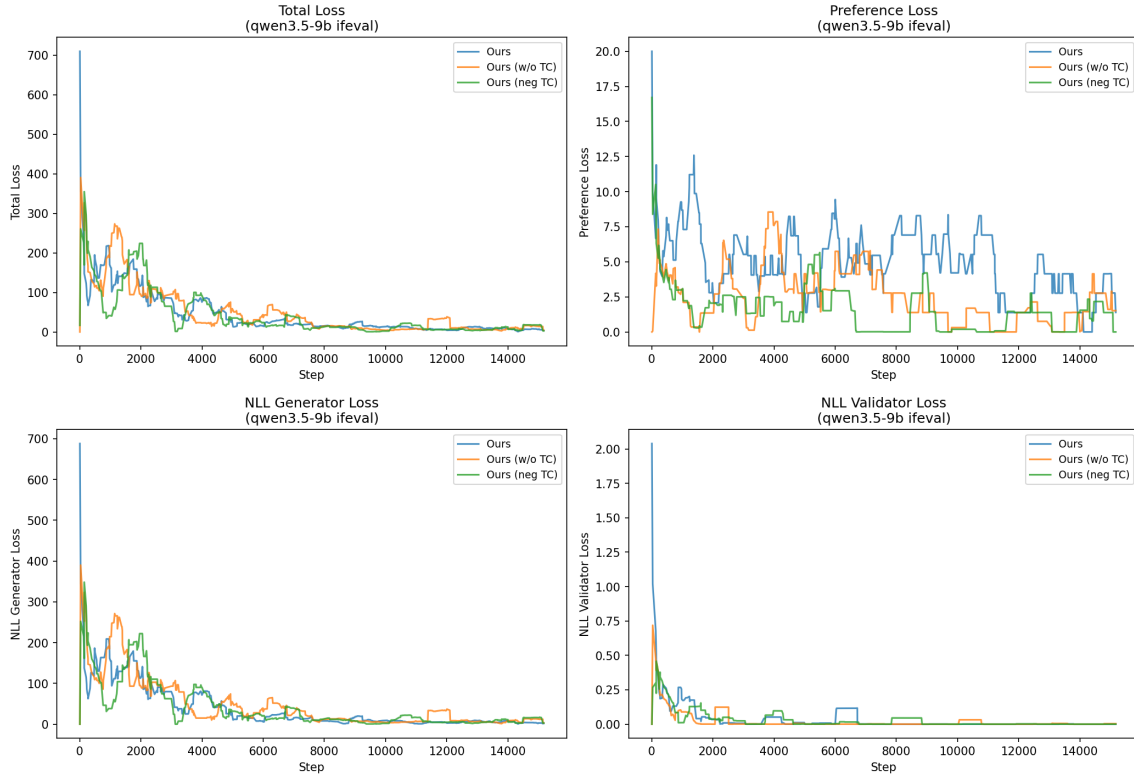
Figure 7: Loss curves: Ours TC comparison (Qwen3.5-9B, IFEval).
