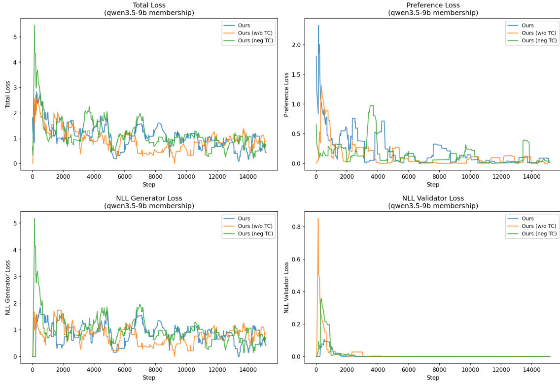
Figure 5: Loss curves: Ours TC comparison (Qwen3.5-9B, membership).
