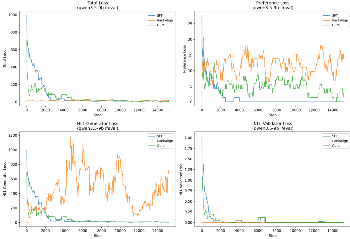
Figure 6: Loss curves: SFT vs RankAlign vs Ours (Qwen3.5-9B, IFEval).
