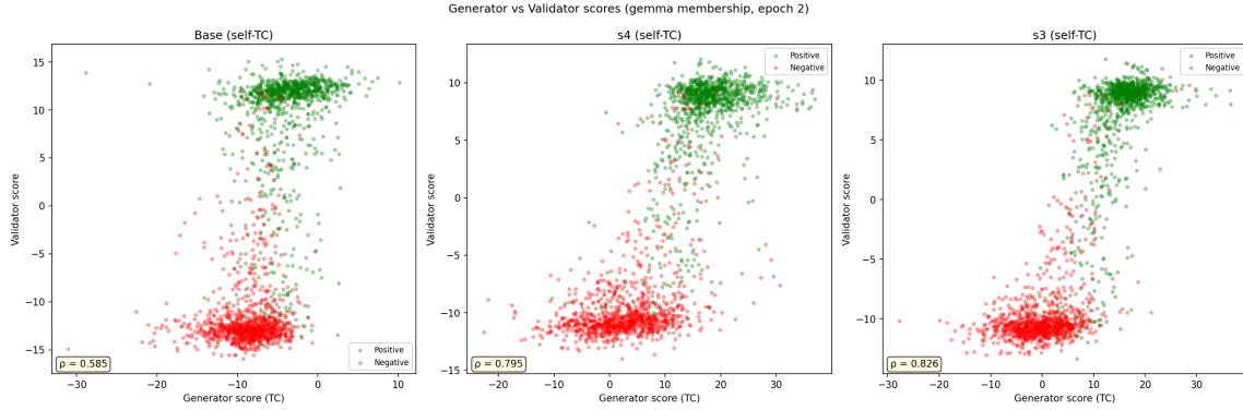
Figure 11: Generator vs validator scores for Base, s4, and s3 (self-TC scoring, gemma membership). Training improves the separation between positive (green) and negative (red) items in both generator and validator space.
