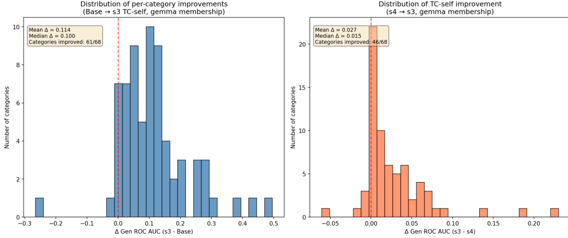
Figure 12: Left: distribution of per-category improvements (Base \rightarrow s3). Right: improvements from TC-self specifically (s4 \rightarrow s3). Both are consistently positive.
