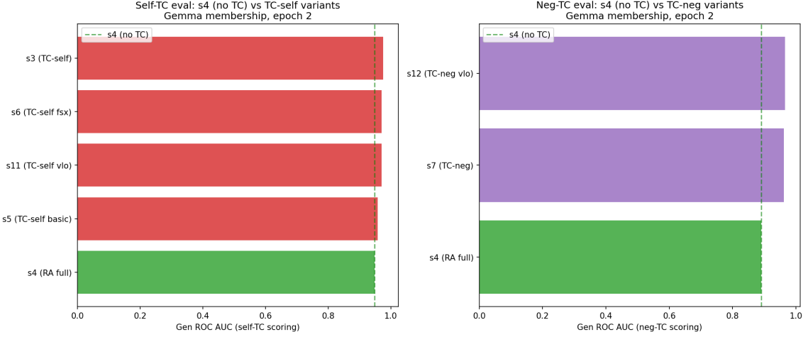
Figure 13: TC comparison: self-TC variants (left) and neg-TC variants (right) against s4 baseline.
