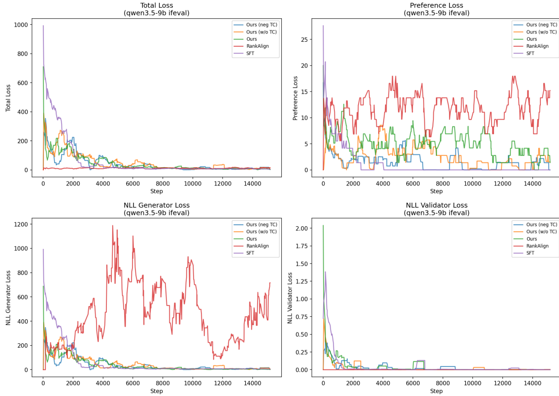
Figure 4: Training loss curves for Qwen3.5-9B on IFEval.
