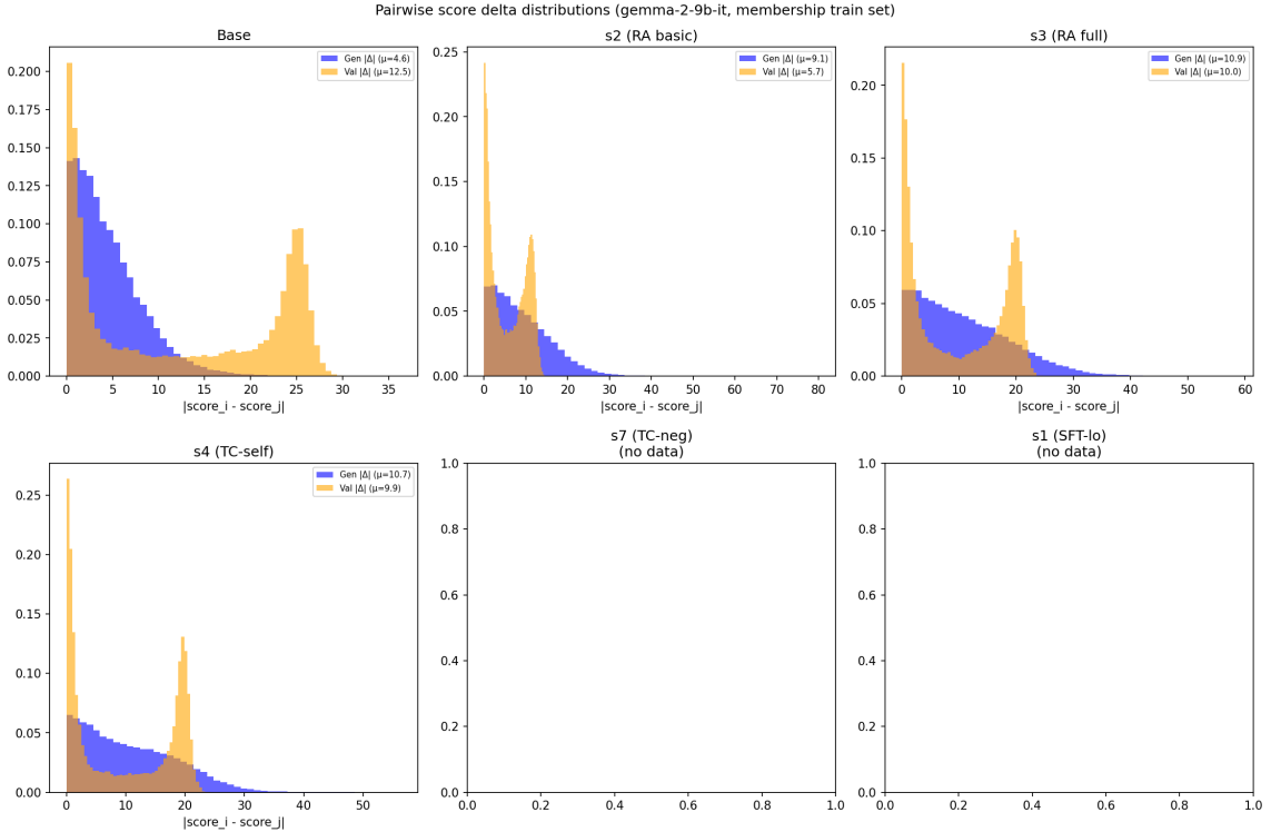
Figure 7: Pairwise score delta distributions for gemma membership. Generator (blue) and validator (orange) distributions. Tighter = better calibrated.
