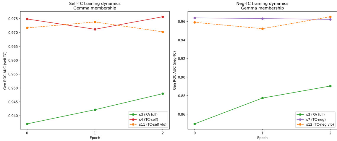
Figure 13: Epoch-by-epoch dynamics for TC comparison. TC-trained models converge quickly and maintain advantage throughout training.
