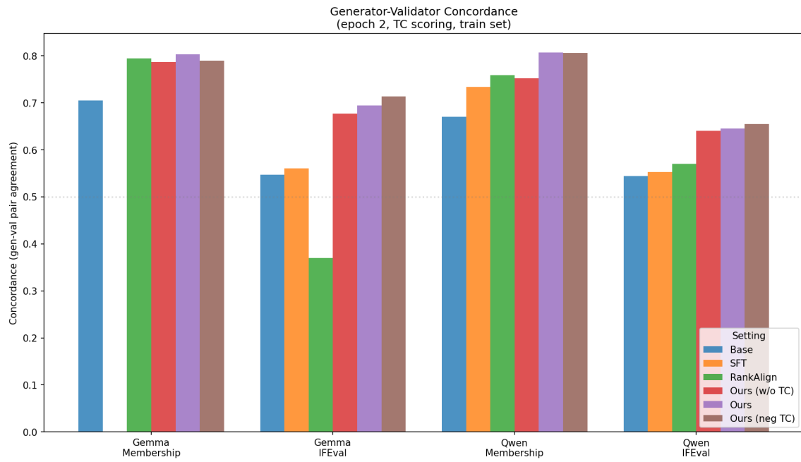
Figure 9: Concordance across all model/task combinations.
