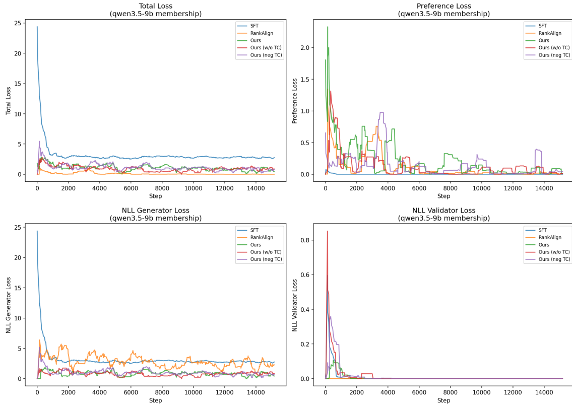
Figure 3: Training loss curves for Qwen3.5-9B on membership.
