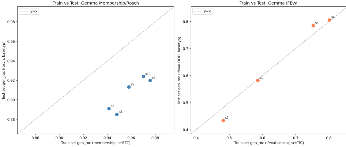
Figure 14: Train vs test set gen_roc. Left: membership train \leftrightarrow rosch test. Right: ifeval train \leftrightarrow ifeval OOD test.
