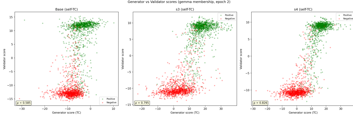
Figure 10: Generator vs validator scores for Base, s3, and s4 (self-TC scoring, gemma membership). Training improves the separation between positive (green) and negative (red) items in both generator and validator space.
