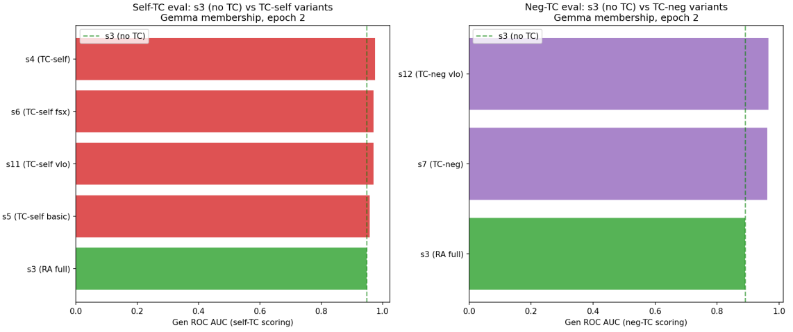
Figure 12: TC comparison: self-TC variants (left) and neg-TC variants (right) against s3 baseline.
