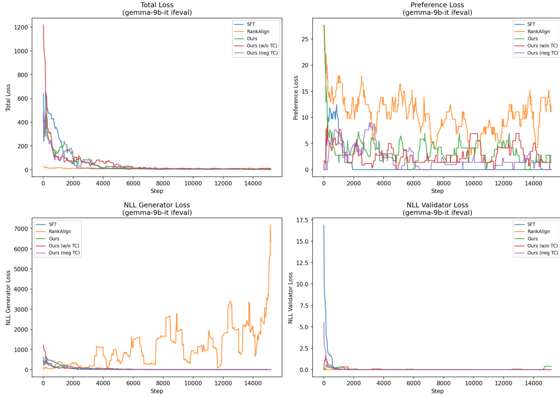
Figure 2: Training loss curves for gemma-2-9b-it on IFEval.
