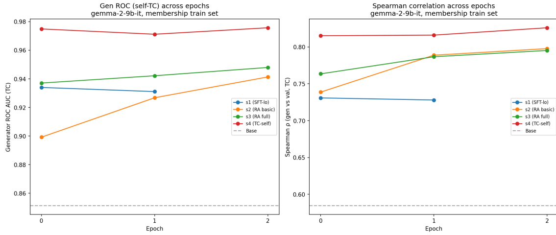
Figure 8: Training dynamics for gemma membership: Gen ROC and Spearman across epochs.
