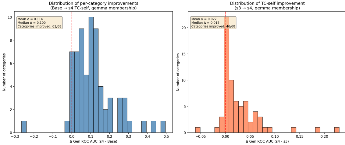
Figure 14: Left: distribution of per-category improvements (Base → s4). Right: improvements from TC-self specifically (s3 → s4). Both are consistently positive.
