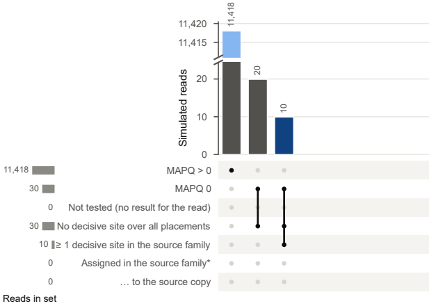
c Gorilla OR6737 (testis, mGorGor1), chr20 (NC_073244.2) catalog: 11,448 simulated reads
