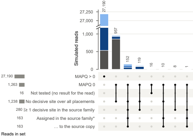
a Human A119b (CHM13 v2.0), chr16 catalog: 28,453 simulated reads
