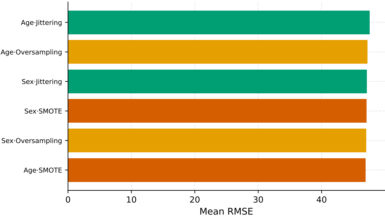
Oversampling: Mean RMSE
