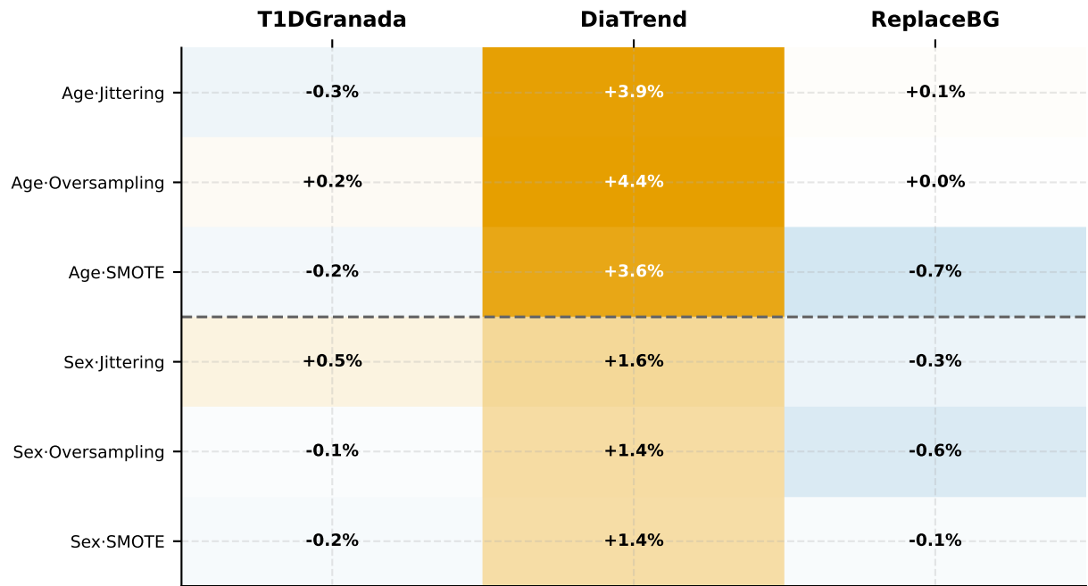
Oversampling: TIR improvement
