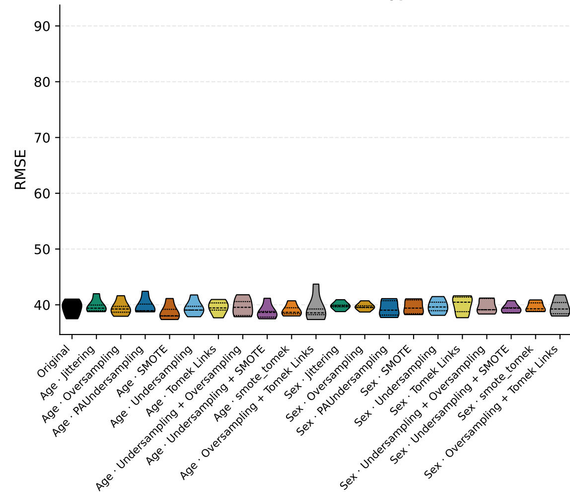
T1DGranada — RMSE · Hypo L2
