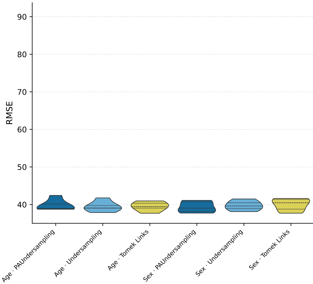
T1DGranada — RMSE · Hypo L2
