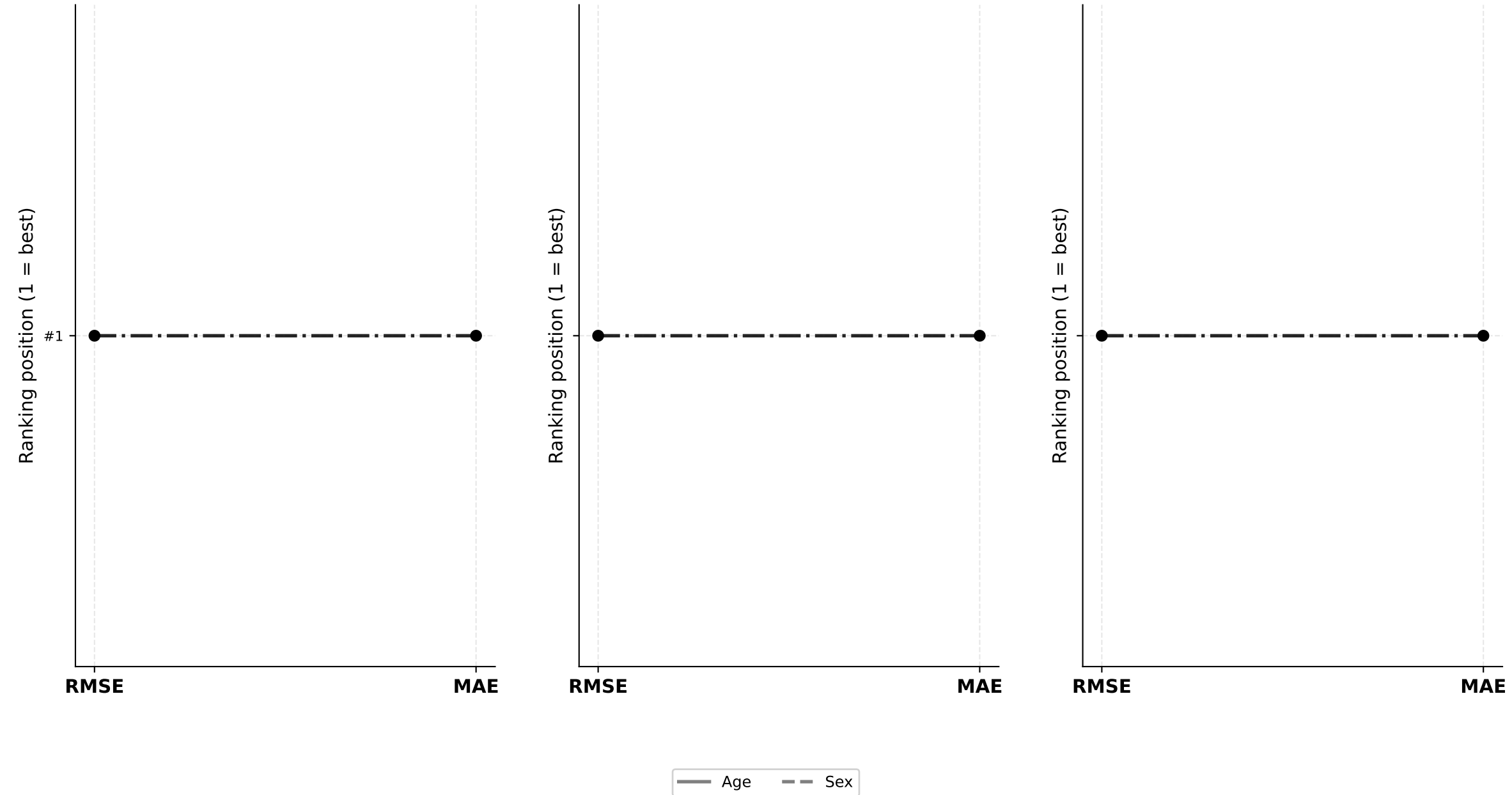
T1DGranada
