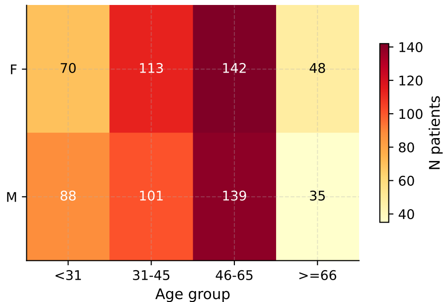
T1DGranada
