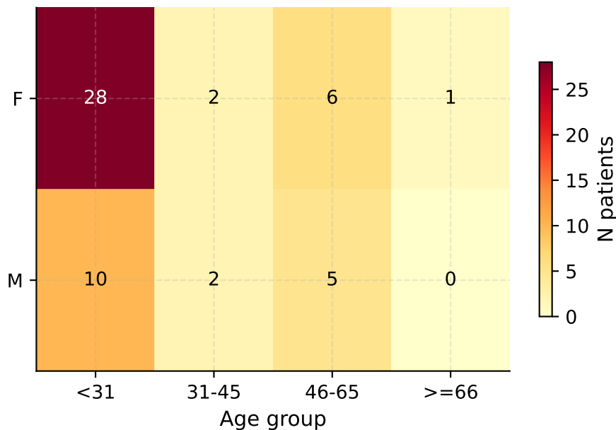
DiaTrend
