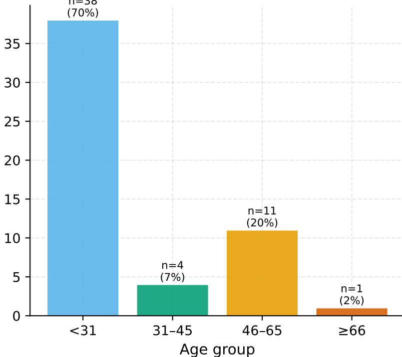
DiaTrend
