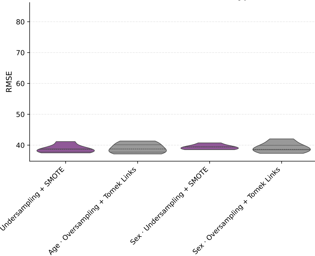
T1DiabetesGranada — RMSE · Hypo L2
