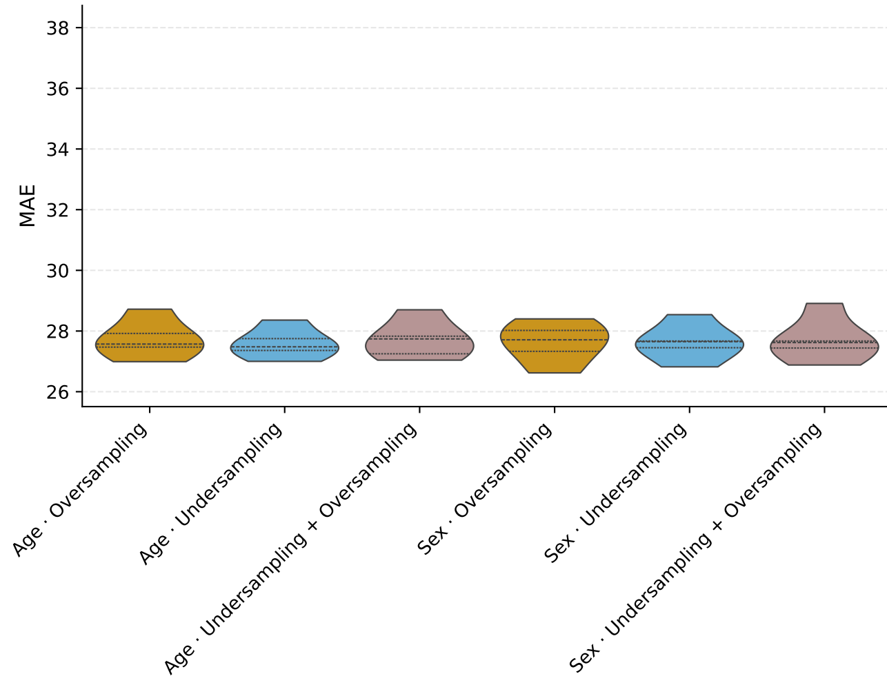
T1DiabetesGranada — MAE · All Ranges
