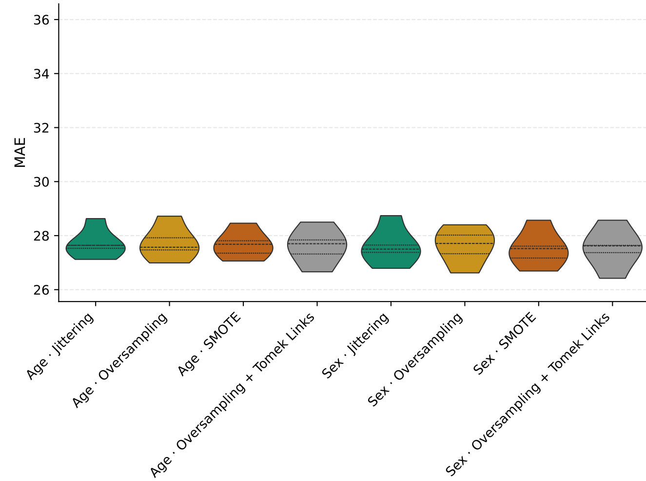
T1DiabetesGranada — MAE · All Ranges
