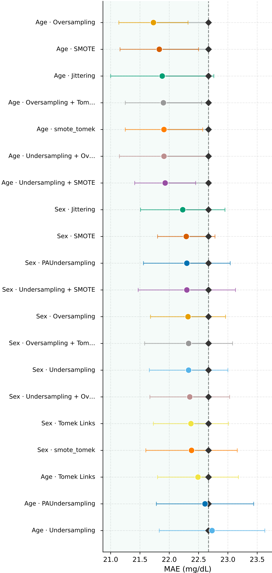
DiaTrend
