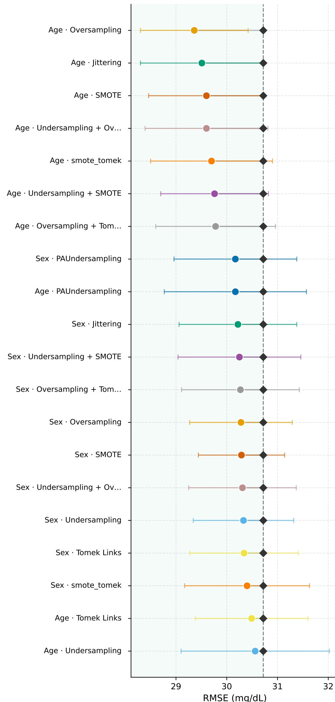
DiaTrend
