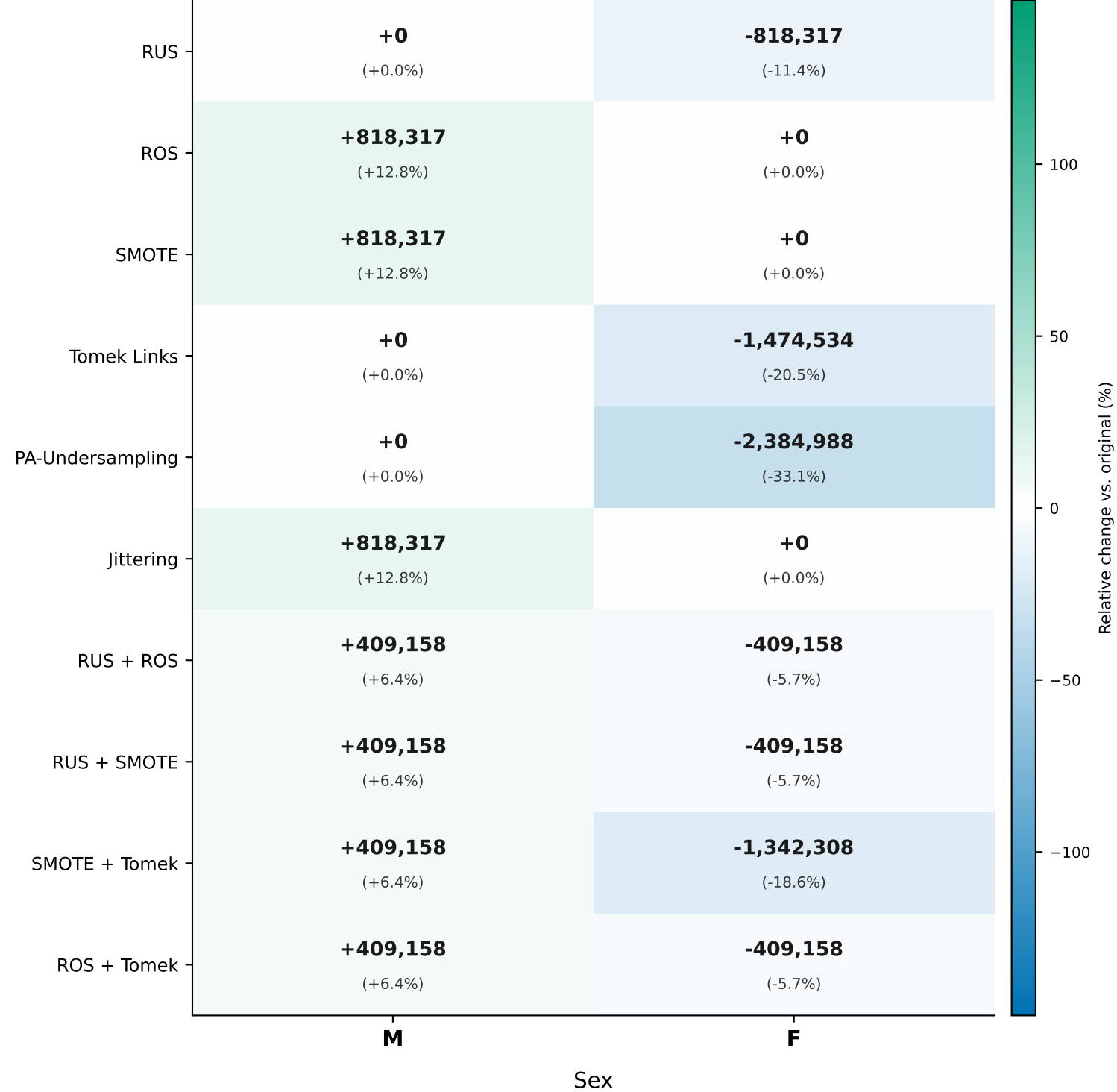
T1DiabetesGranada · Balancing effect on train composition (Sex dimension) Cell: mean \Delta samples (bold) and \Delta\% across 5 folds | Blue = loss · Green = gain
