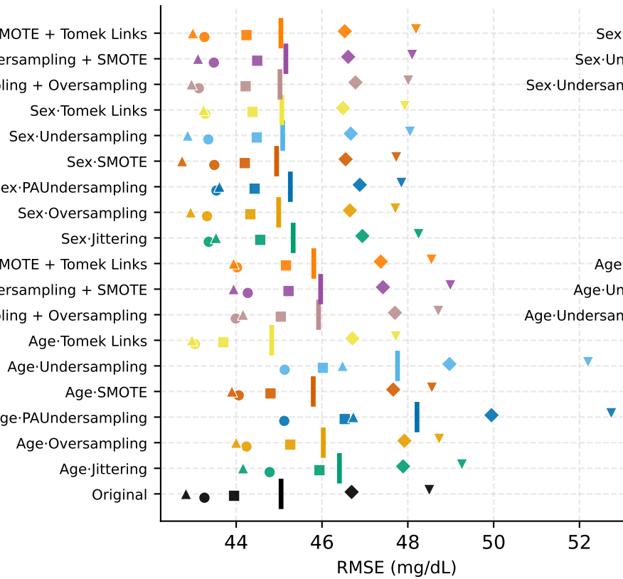
Fold consistency — | = mean
