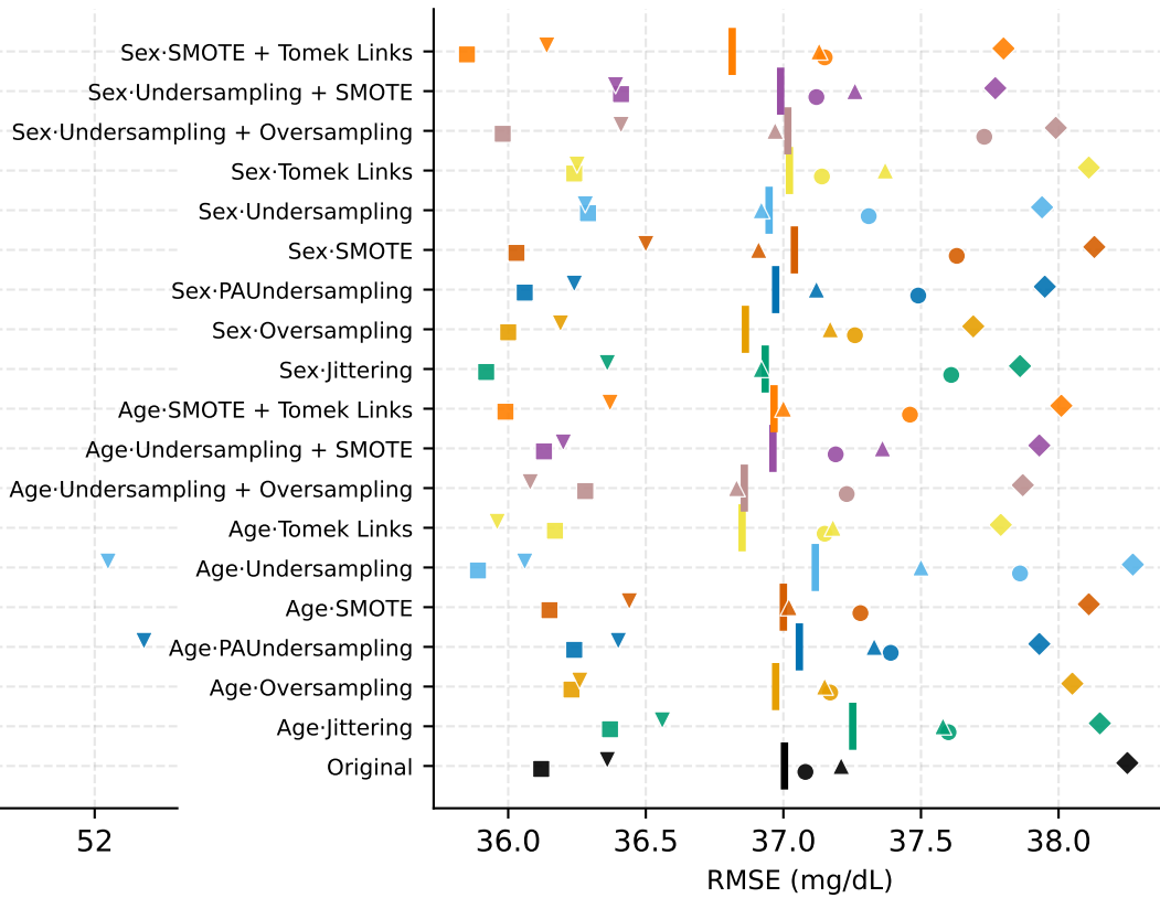
Fold consistency — | = mean
