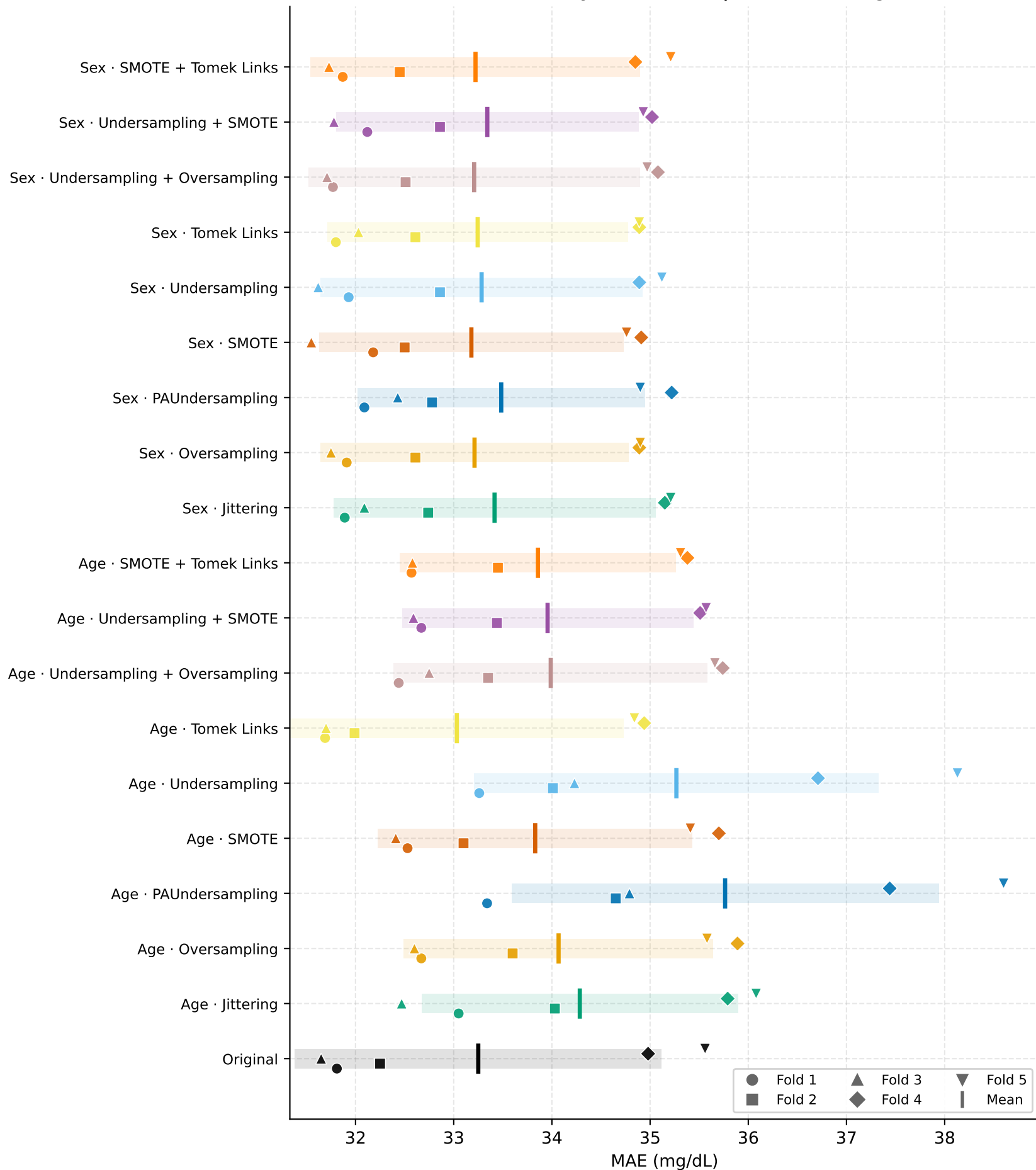
Fold consistency — DiaTrend | MAE · All Ranges
