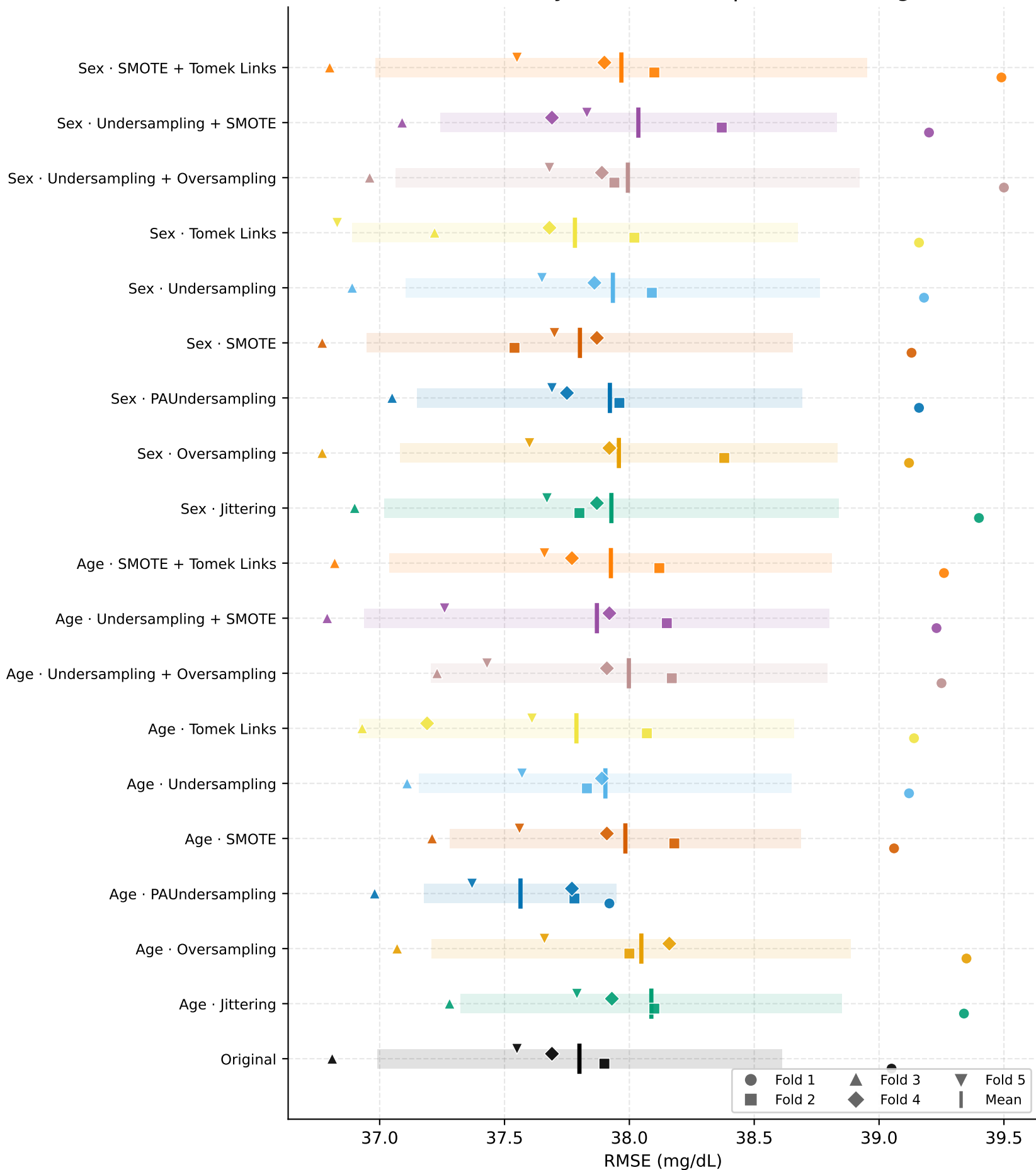
Fold consistency — T1DGranada | RMSE · All Ranges
