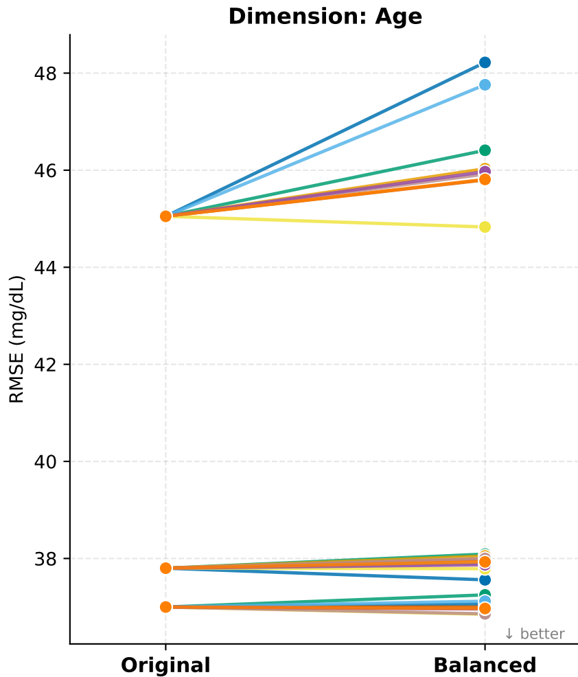
Slope chart — RMSE · All Ranges
