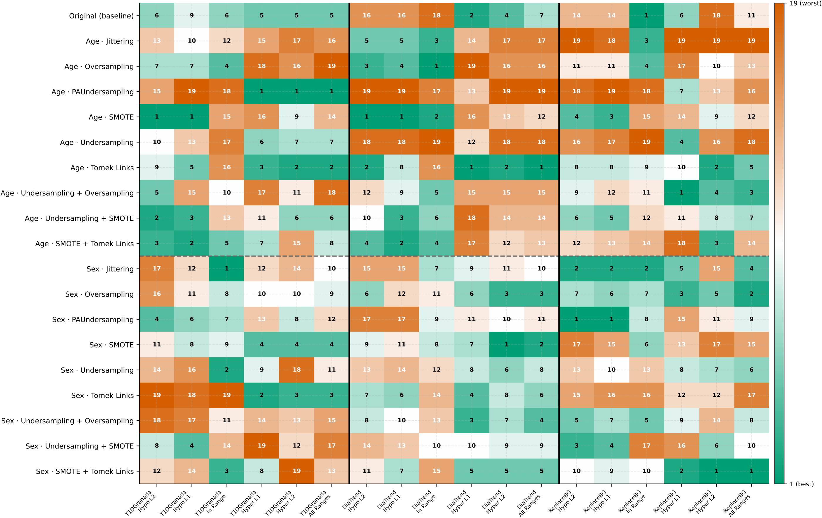
Ranking position by technique × dataset × glucose range | MAE
